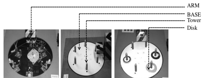
FIGURE 2: LAYOUT FOR CIRCUIT AND OTHER COMPONENTS OF HANOI
