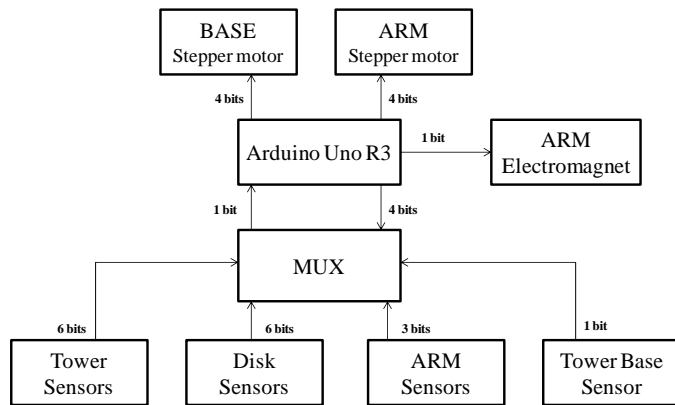
FIGURE 3: BLOCK DIAGRAM OF BITWISE OPERATION
