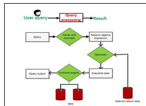
Figure 1: The query processing process
