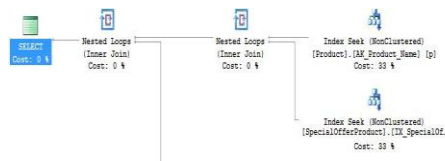
Figure 5: Query plan join three table methods
