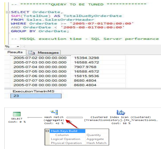
Figure 3: query plan and query execution time for aggregation method
