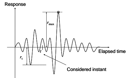
Figure 4. Maximum seismic responses within a given elapsed time and duration of an earthquake.
