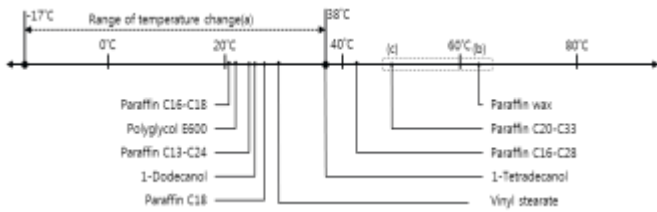
Figure 2. Selection of Paraffin Considering Temperature Change
