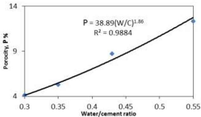
Figure 2: relationship of porosity with water-cement ratio
