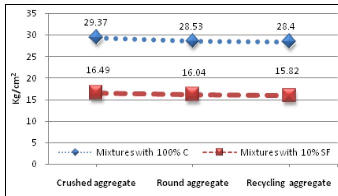
Figure 6. Flexural strength of pervious concrete.
