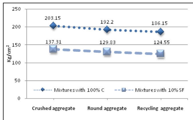
Figure 7. Compressive strength of pervious concrete.
