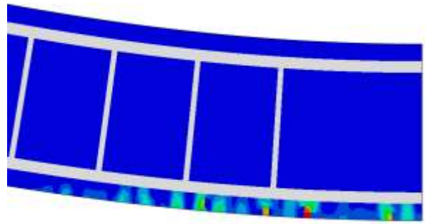
Figure 12. Tensile damage at middle of interior span using 30% of A_s'
