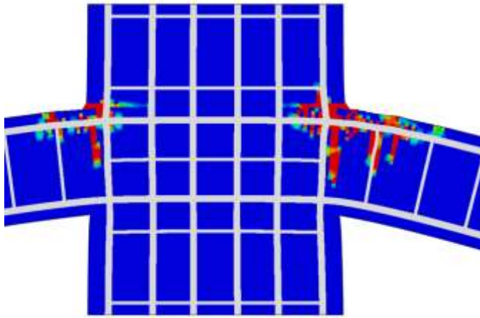
Figure 10. Percentage of compression steel at midspan, 30%
