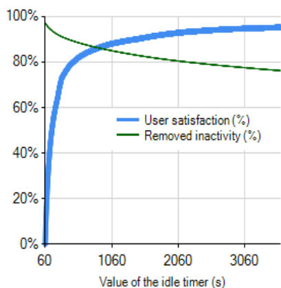
Figure 7. Zoom of curves of user satisfaction and removed inactivity for low values of the idle timer
