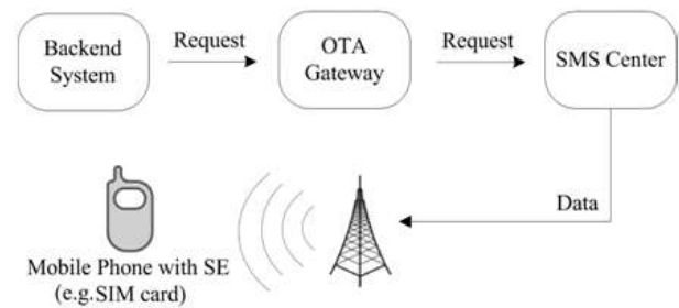
Figure 3. Basic OTA architecture
