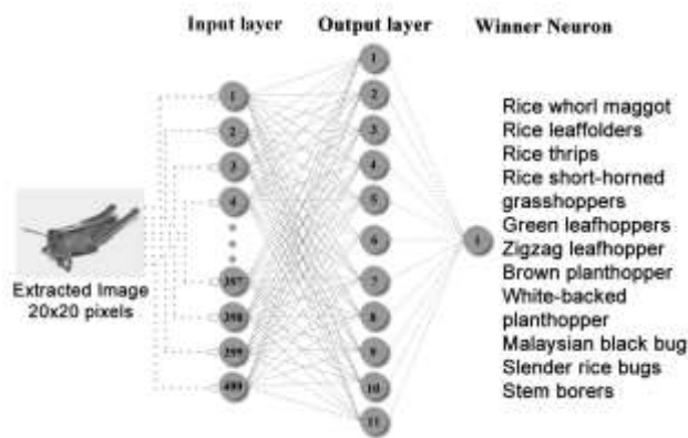
Figure 3. Neural network design for pest identification
