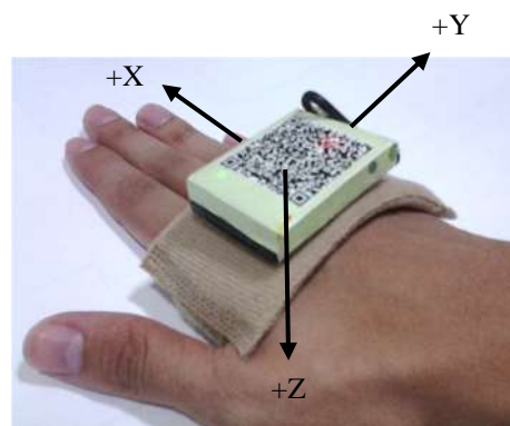
Figure 1. Wearable sensor device
