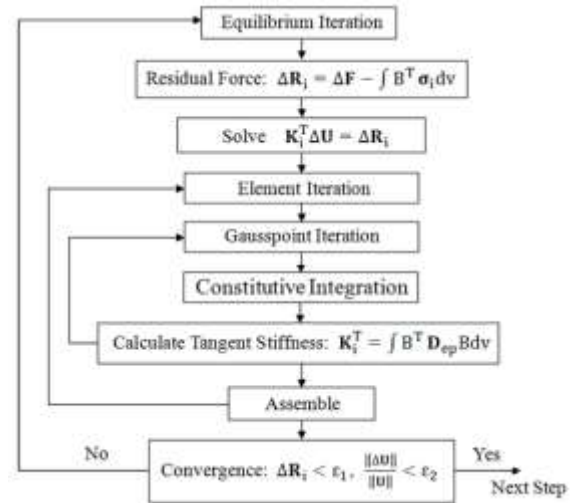
Figure 4 Algorithm for structure in one step
