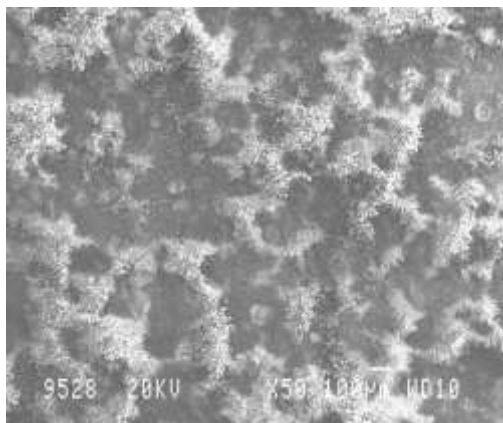
Figure 10. Wear track of neat epoxy with 15N and 250m of 150 grit size (a) 50X
