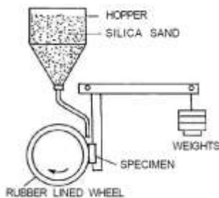
Figure 6. Schematic diagram of dry sand/rubber wheel abrasivewear test rig
