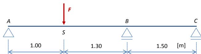
Figure 5. Experiment layout.
