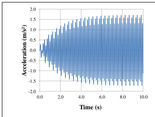
Figure 6. Floor dynamic reponse for 64 persons.Nodes G and K. Time domain. Dynamic loading model I.
