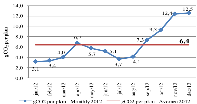
Figure 2. Emissions, in gCO 2 per pkm, from Rio de Janeiro Subway - 2012
