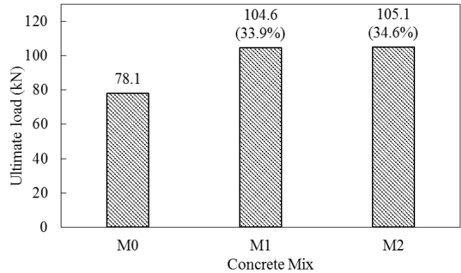
Figure 6. Ultimate load capacity of control and SFRC slabs.
