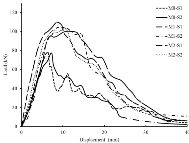
Figure 5. Load-displacement variation for punching of RC and SFRC slabs.
