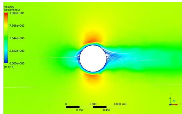
Figure 2: Velocity surface streamline
