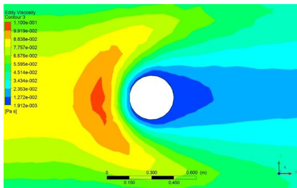
Figure 6: Eddy viscosity contour
