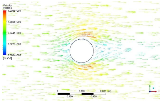
Figure 3: Velocity vector
