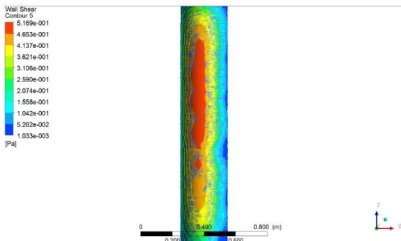
Figure 13 : Wall Shear Contour
