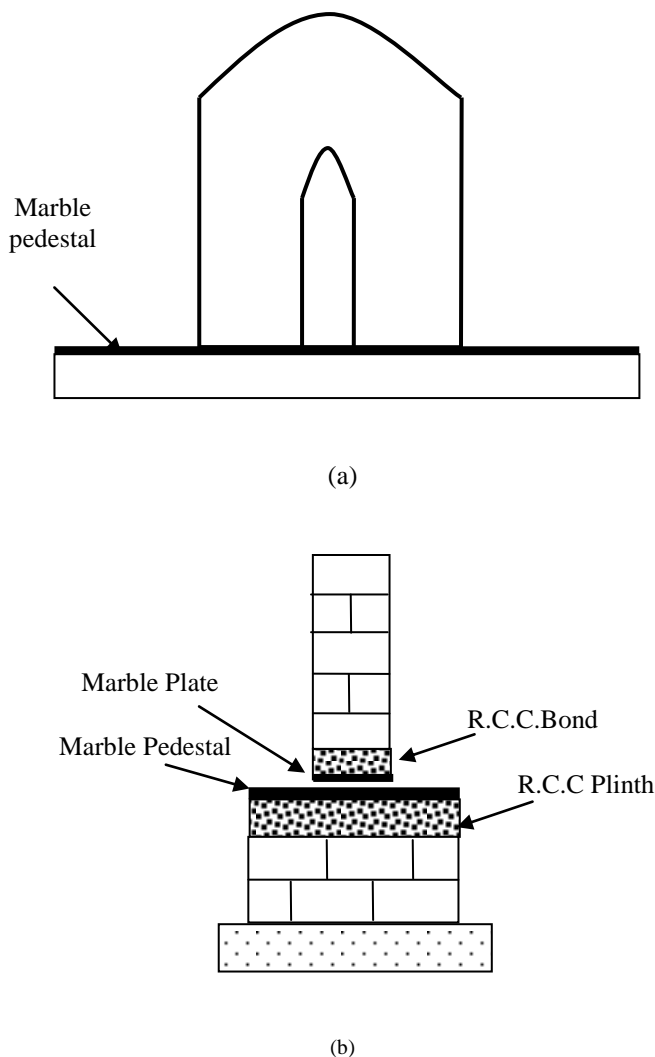
Figure 1. Construction detail for frictional base-isolation system for architectural temples with (a) large marble pedestal and (b) wall section.
