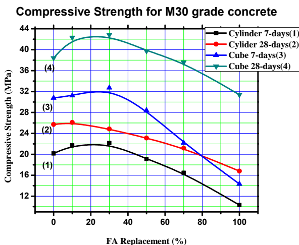
Figure 4. Variation of Cube & Cylinder Compressive Strength (M30)
