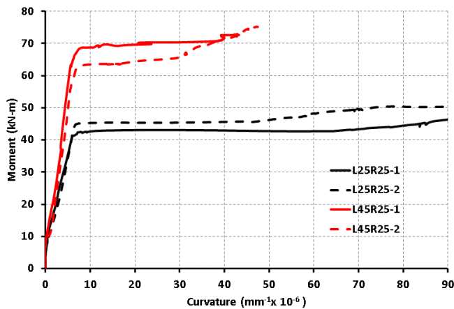
Figure 3. Moment-Curvature curves for LWC beams with \rho = 0.25 \rho_{bal} and varying concrete strengths.
