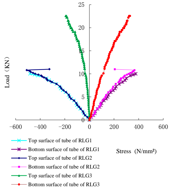
Figure 3. Load-stress curve
