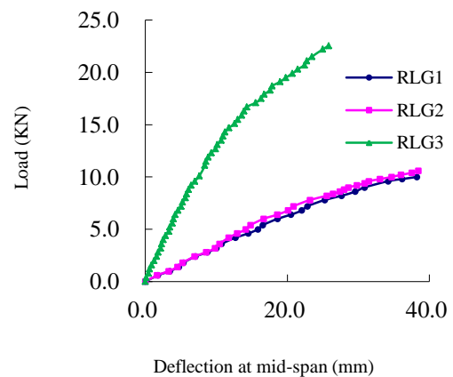
Figure 4. Load-deflection curve
