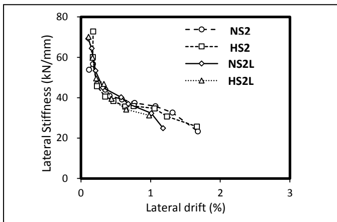
Figure 4. Stiffness degradation curves
