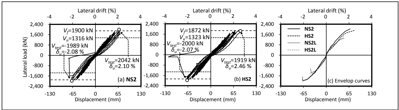
Figure 3. Load-displacement relationships and envelop curves
