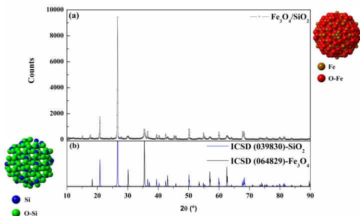
Figure 4. (a) Diffratogram of Fe 3 O 4 particles supported on SiO 2 . (b) indexation of crystalline plans corresponding to SiO 2 and Fe 3 O 4 , accompanied by the representation of the clusters for each structure.
