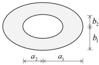
Figure 2. Elliptical hollow cross-section.
