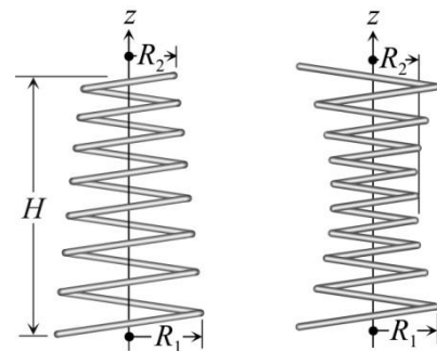
Figure 1. Conical and hyperboloidal helix geometry.
