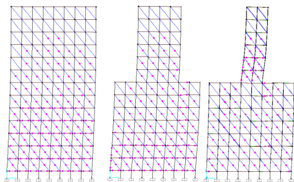
Figure 8 Hinge pattern at yielding for (a) R, (b) IR1, (c) IR2
