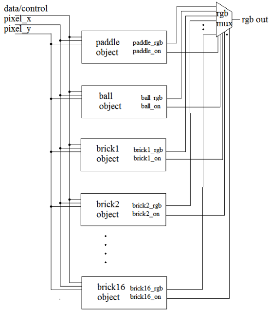
Figure 5. Object-mapped scheme
