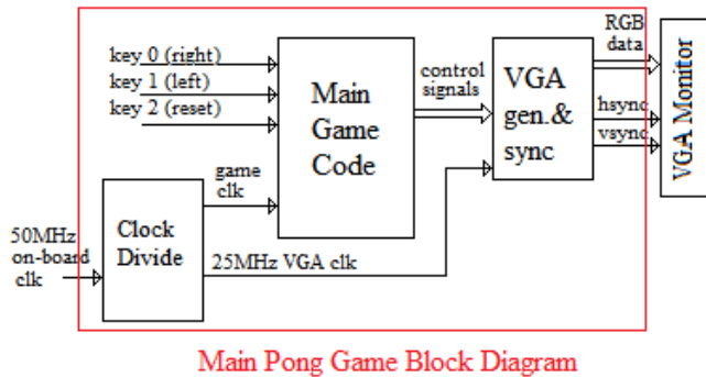
Figure 3. Main block diagram of the VHDL Pong Code
