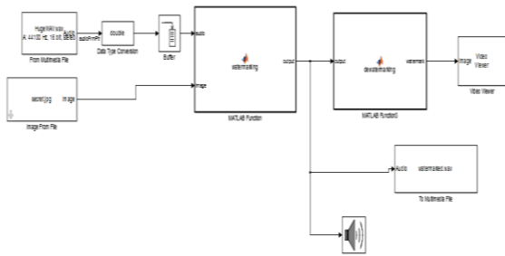
Figure 2. Simulation block for watermarking insertion and extraction
