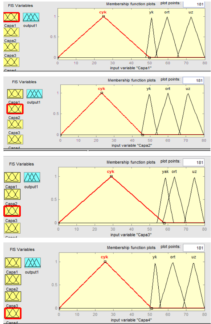
Figure 5. The input and output membership functions for each anchors
