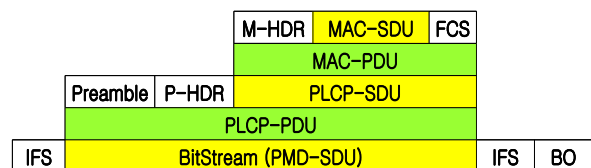
Figure 1. Protocol stack of physical and MAC layer
