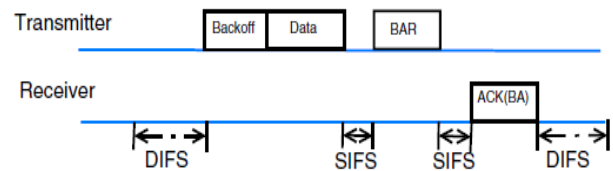
Figure 2. Basic access scheme[10]
