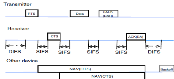
Figure 3. RTS/CTS access scheme[10]
