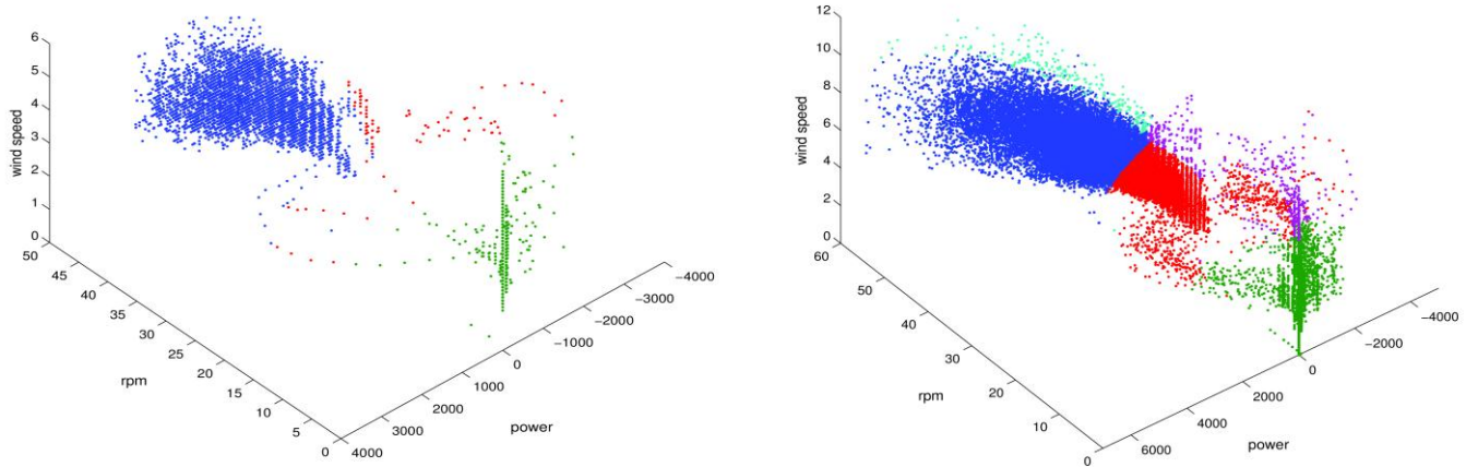
Fig.2. Operational states classification of the vertical axis wind turbine data by the system of the ART-2 neural network and the stereographic projection normalization. The left plot shows starting 10.000 data points of a full data set (500.000 points) placed in the right plot.
