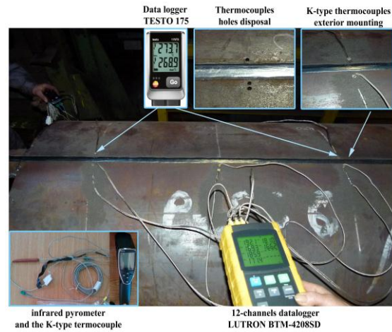
Figure 4. Temperature measurement system outside the pipeline
