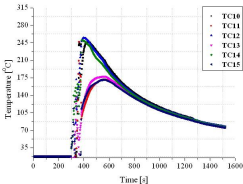
Figure 7. Temperature vs. time recorded by the thermocouples positioned outside the pipeline
