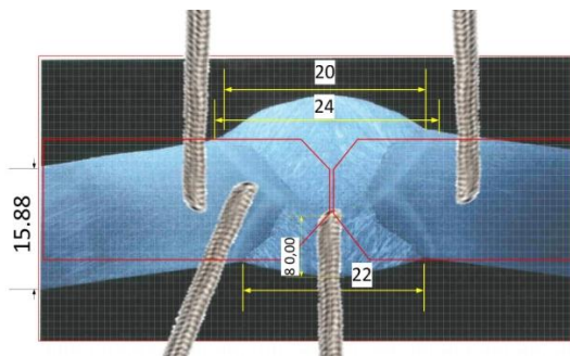
Figure 1. The disposal of thermocouples in the weld and HAZ [6]
