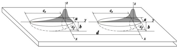
Figure 1. Sketch of heat sources positioning on sheet [5]
