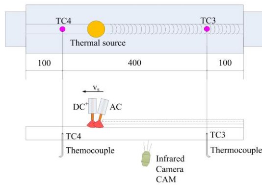
Figure 7. TC3 and TC4 thermocouples arrangement
