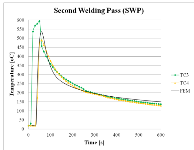
Figure 8. Temperature vs. time in TSAW process
