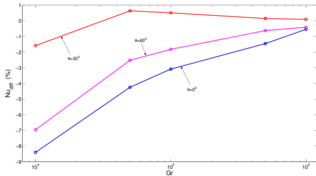
Fig.4 Difference between averaged heat transfer for cylinder and no-cylinder configurations for various Grashof numbers ( Ha=30 , \phi=0.02 )
