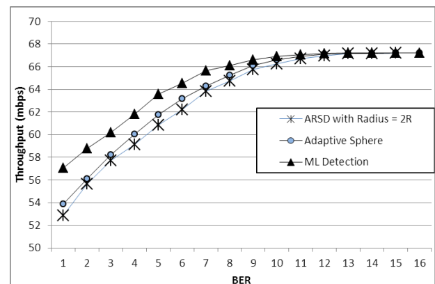
Figure 7. Throughput Vs. SNR curve for ARSD-K Best algorithm
