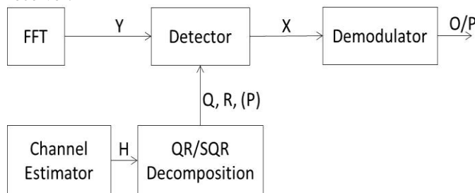
Figure 1. Block Diagram of the MIMO receiver
