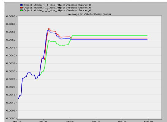
Figure 7. Average delay for rtPS users
