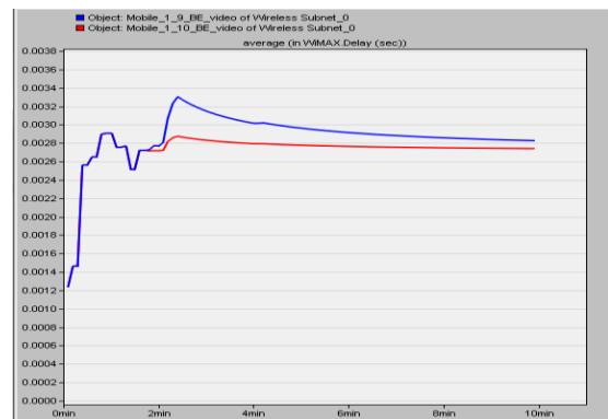
Figure 6. Average delay for BE users
