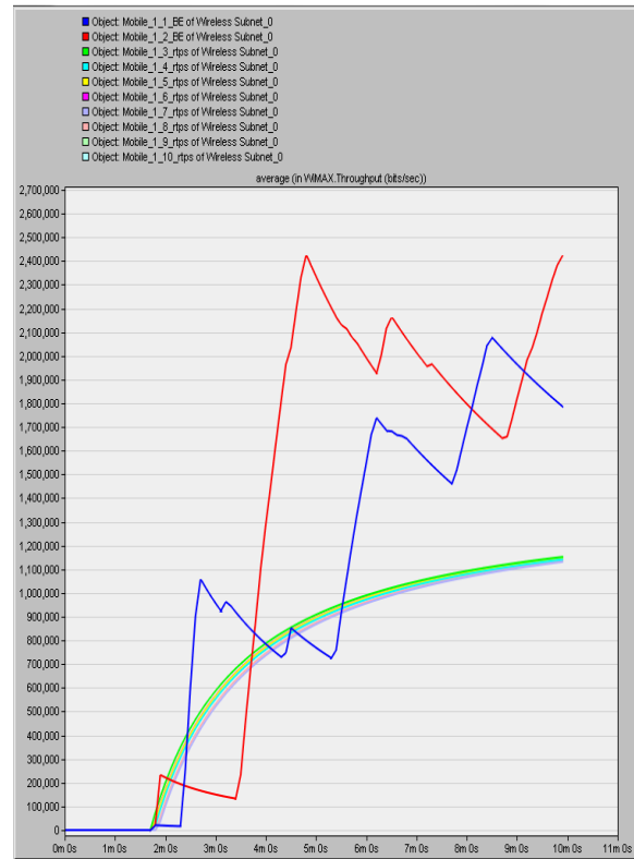
Figure 2. Average throughput for rtPS and BE
