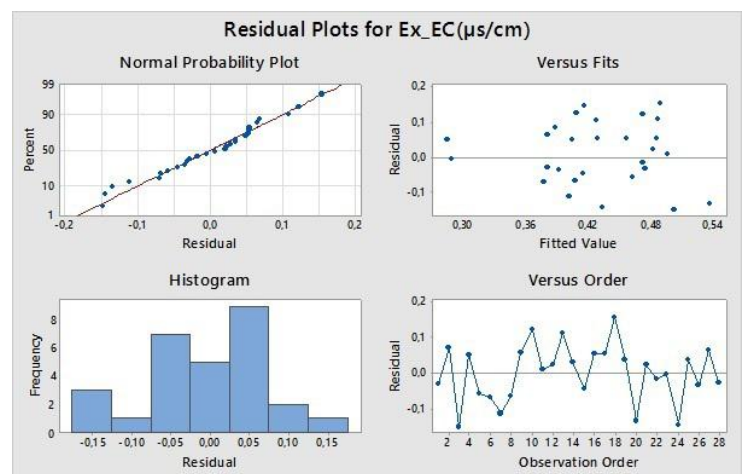
Figure 5. Residual Plots
