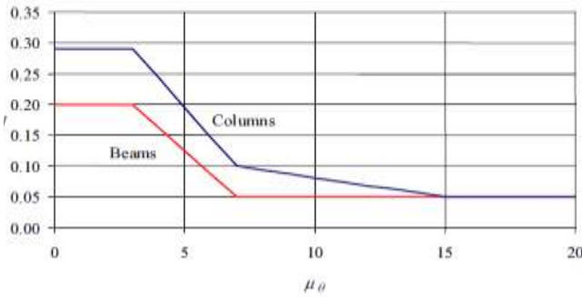
Figure 1. Shear strength degradation coefficient for beams and columns [6]
