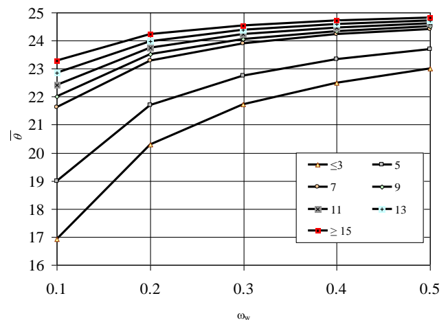
Figure 4. Columns ( n=0.2 ): \bar{\theta} Slope vs. transversal reinforcement mechanical ratio for different values of flexural ductility demand
