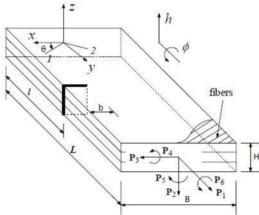
Figure 14 Fibre reinforced composite beam geometry [7]
