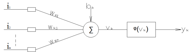
Figure 6 Neuron architecture
