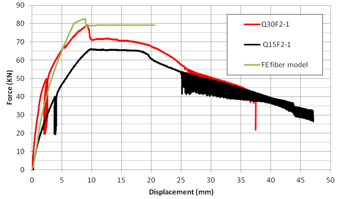
Figure 10. Fiber FE models: predicted force-deflection
