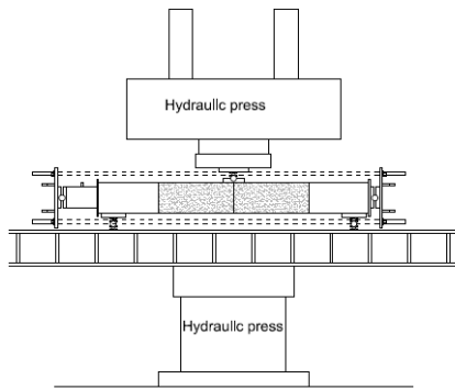
Figure 6. Test setup for three point bending test
