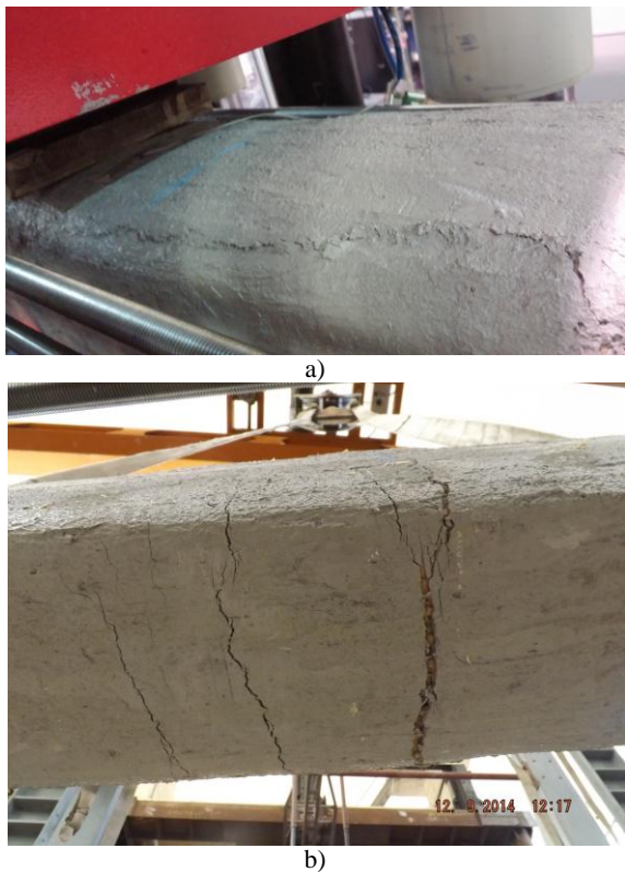
Figure 11. Q30F2-1 specimen at the test end: a) top face; b) bottom face
