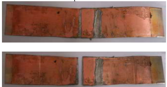
Figure 2: Failure Modes of Lap-Shear Specimens
