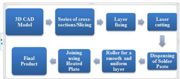
Figure 1: Composite metal foil manufacturing process
