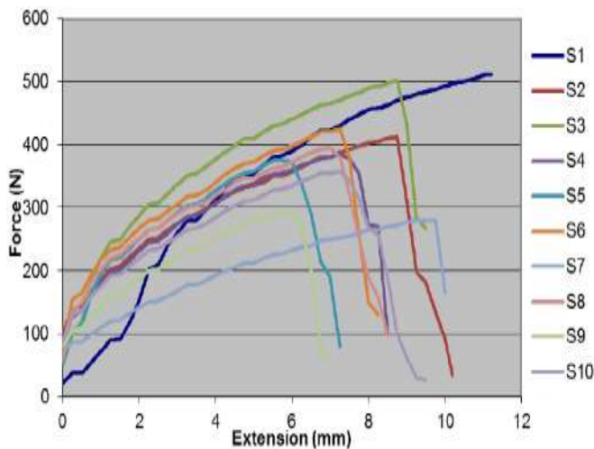
Figure 3: Lap-shear test results
