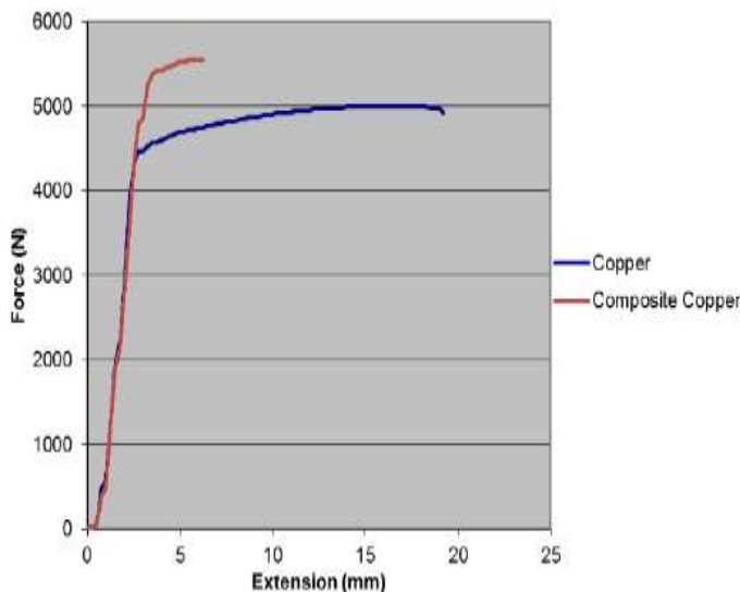
Figure 3: Comparative tensile test results
