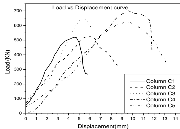
Figure 5. Load vs, Displacement curves of columns
