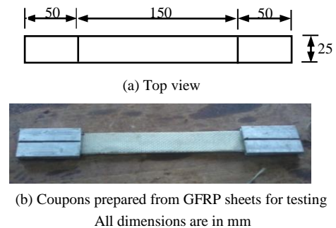
Figure 1. Details of GFRP coupons
