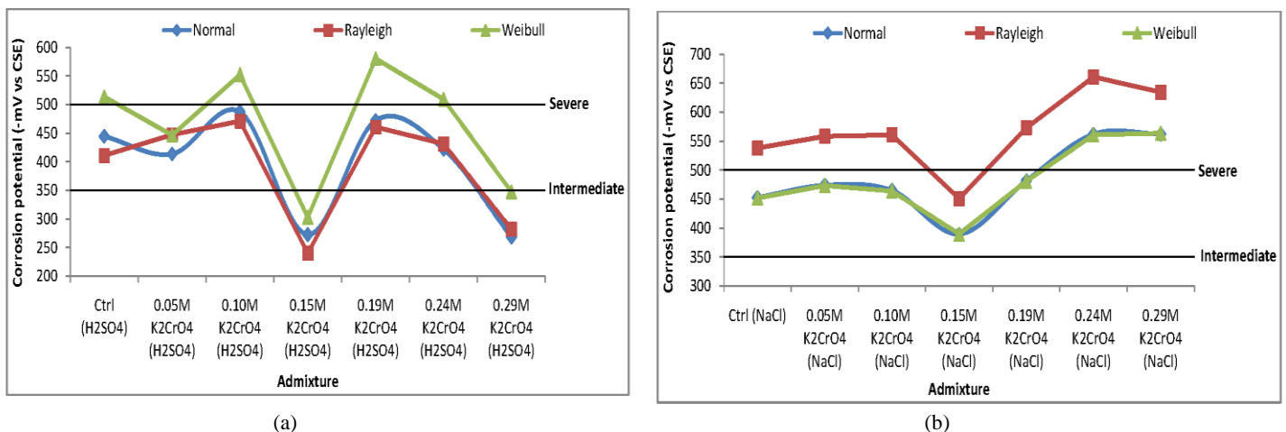
Fig. 1. Plots of statistical distribution predictions of mean corrosion potential in steel-reinforced concrete samples with linear plots of corrosion risk/probability as per ASTM C876-91 R99 [8-9,22]
