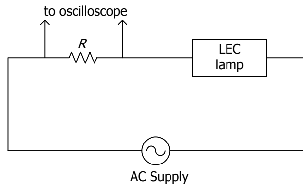
Figure 3. Equivalent circuit of the system
