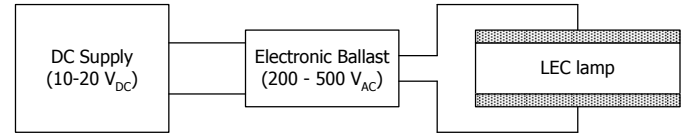
Figure 2. Diagram of electrical connection
