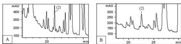
Figure 5 The chromatograms of carbaryl in the sample solution before (A) and after (B) SPE clean up step. Peak identification: (2) carbaryl.
