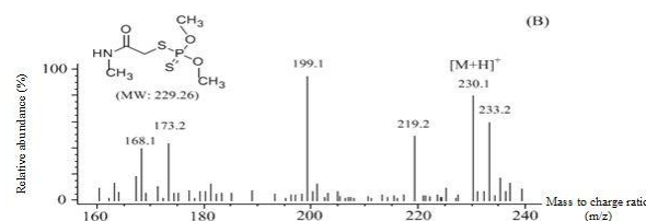
Figure 8 The mass spectrum of dimethoate.
