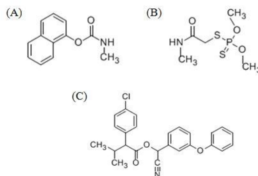
Figure 1 The structures of (A) carbaryl (B) dimethoate (C) Fenvalerate.
