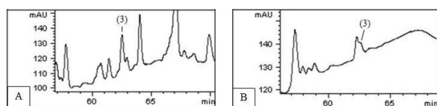
Figure 6 The chromatograms of fenvalerate in the sample solution before (A) and after (B) SPE clean up step. Peak identification: (3) fenvalerate.
