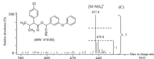
Figure 9 The mass spectrum of fenvalerate
