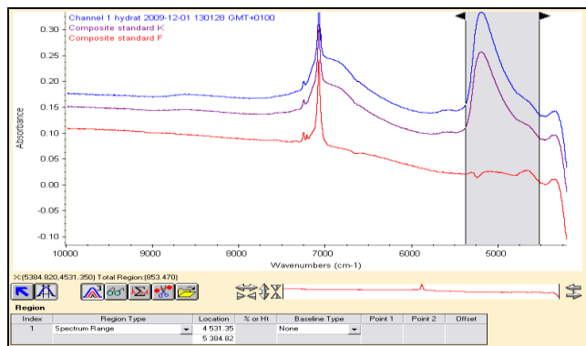
Figure 1. Comparison of NIR spectras of lime hydrate as the function of moisture contents (taken from the NIR device screen)
