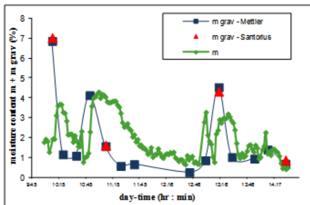
Figure 3. Comparison of moisture-Content measurement by the "conventional" and the NIR spectral methods.
