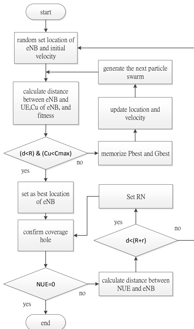
Figure 3. PSO Flowchart
