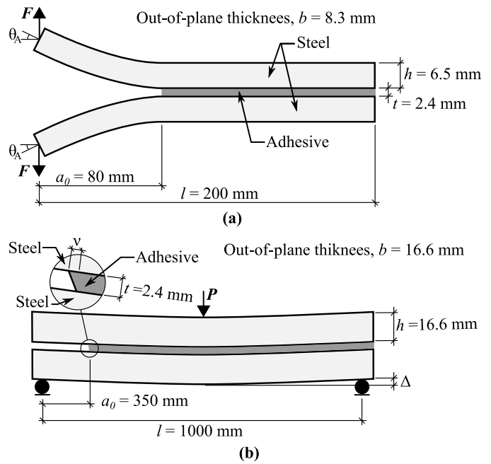
Figure 1. Geometry of specimens used in this study: (a) DCB, (b) ENF.
