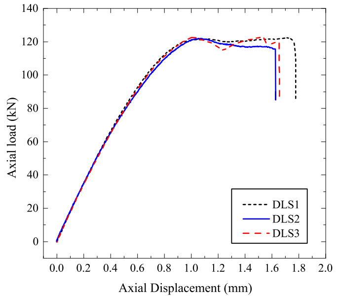
Figure 4. Double lap shear specimens test results
