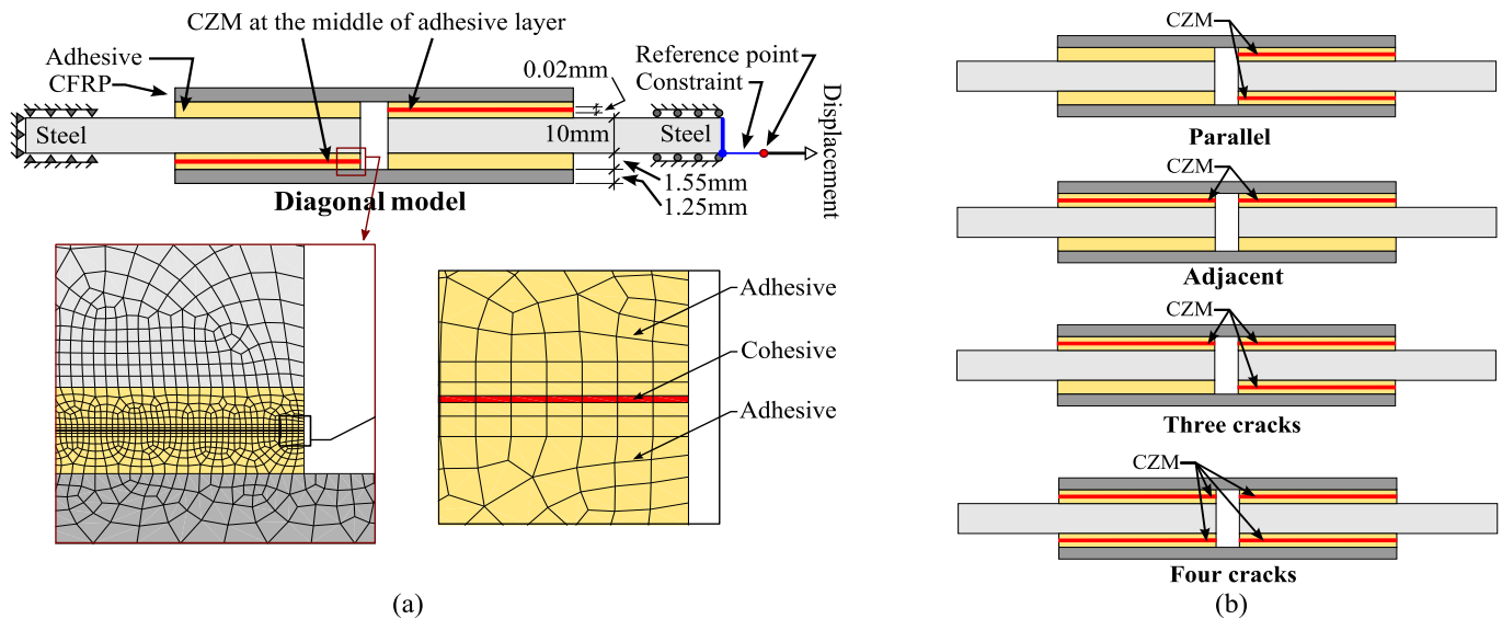
Figure 6. (a) The boundary conditions and general mesh of the DLS joints, (b) different investigated failure modes.
