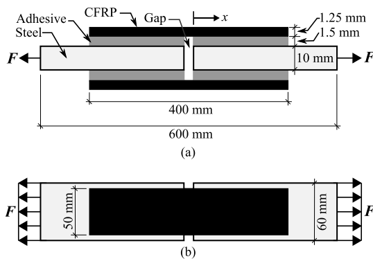
Figure 3. DLS joints: (a) side-view, (b) top-view
