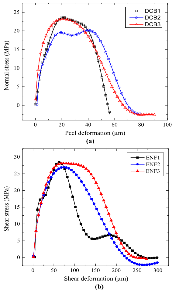
Figure 2. Cohesive laws for the adhesive loaded in (a) mode I, (b) mode II.
