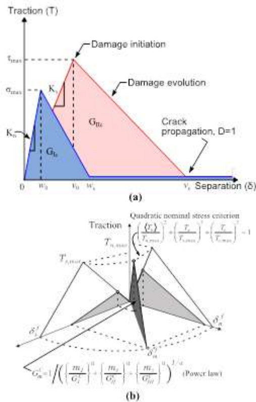
Figure 5. (a) Bilinear cohesive law, (b) CZM mixed mode in ABAQUS™.
