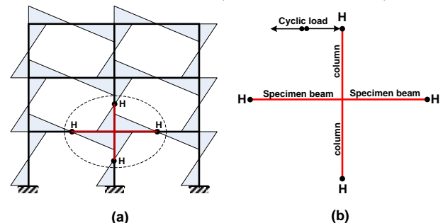
Figure 1. (a) The moment area of a frame due to earthquake loads, (b) Principle of the test beam-column element
