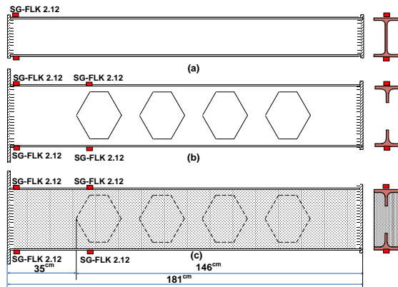
Figure 2. Beam test for the : (a) normal beam (nb), (b) castella (cb), (c) castella composite beam (ccb)
