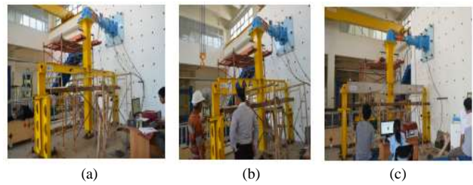
Figure 4. Testing implementation for the, (a) NB test beam, (b) CB test beam and (c) CCB test beam
