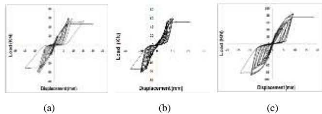
Figure 5. The load-displacement curve relationship (P-Δ) for, (a) NB test beam , (b) CB test beam and (c) CCB test beam
