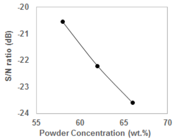
Figure 3(a): Response for S/N ratio corresponding to Powder Concentration
